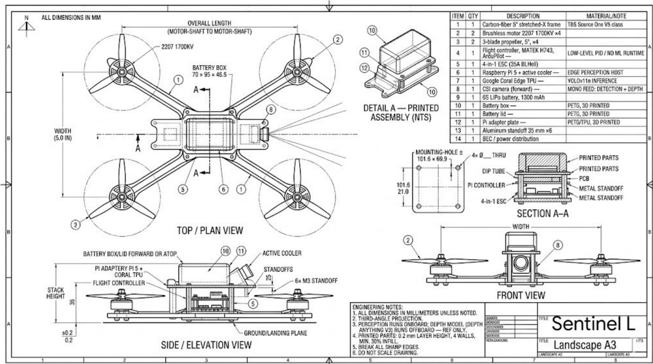
Figure 13. The SENTINEL-Lite aerial platform (“Sentinel L”). A 5-inch stretched-X carbon-fiber quadcopter (2207 1700 KV motors, MATEK H743 flight controller) carrying an onboard Raspberry Pi 5 with a Google Coral Edge TPU for real-time YOLOv11n inference, a Raspberry Pi Camera Module 3 Wide for visible-spectrum imaging, and a Raspberry Pi NoIR Camera Module V2 (8MP, 1080P30) for near-infrared capture, enabling low-cost field screening of water bodies before escalation to the full multimodal cascade. Top/plan, side/elevation, and front views plus printed-assembly detail and section A-A; dimensions in mm.
